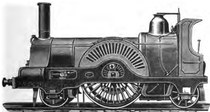
Fig. 62.—Express Engine, built by Neilson, 1862.
